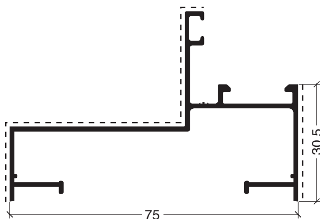
ADR 1176 Marco 75 mm 0,700 kg/m - L = 6170 mm.
