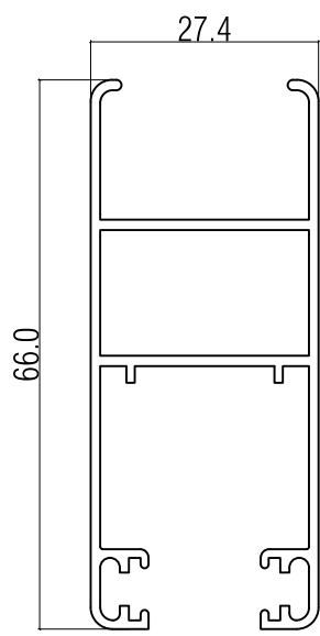
ADR 425 0.697 KG/M
