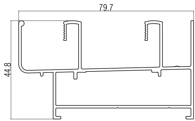
ADR 1510 1.021 KG/M
