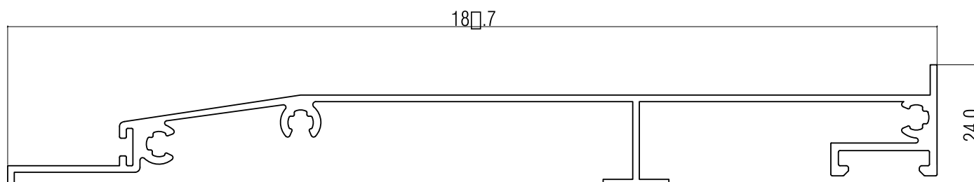
ADR 18615/180mm 1.208 KG/M
