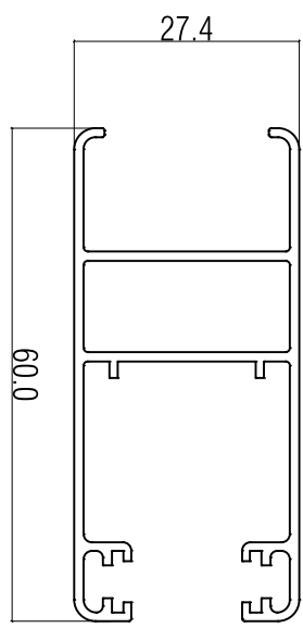
ADR 1650 0.647 KG/M
